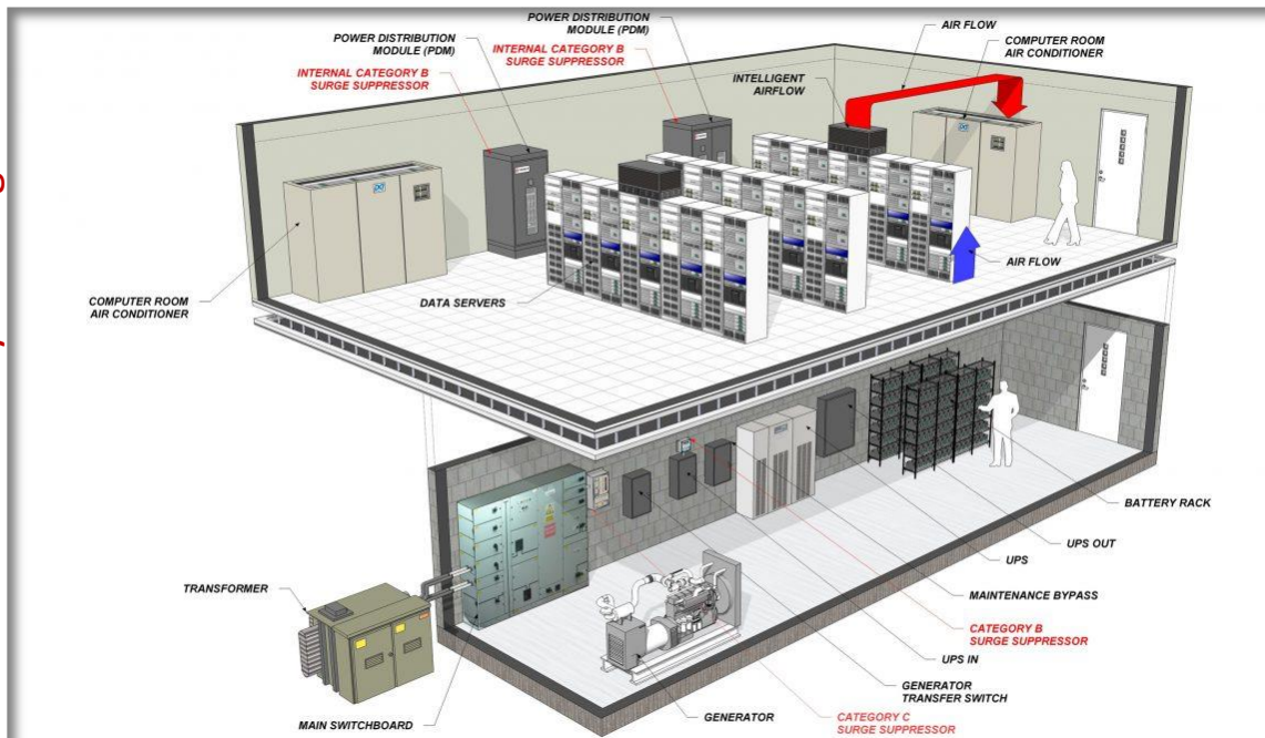
Data Center Layout Diagram
